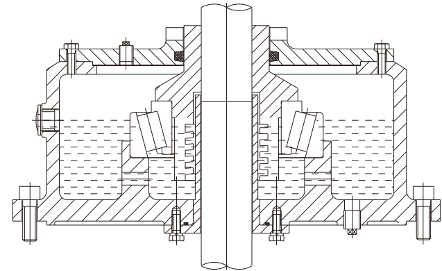
Standard thrust bearing assembly set
